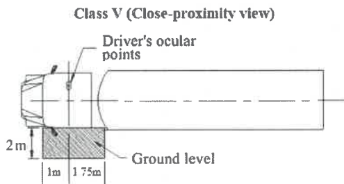
Figure 11 – Minimum required fields of vision for goods vehicles over 3.5 tonnes maximum mass (note: class VI is optional for goods vehicles \leq 7.5 tonnes) (source: adapted (for right-hand-drive) from UN R46)
