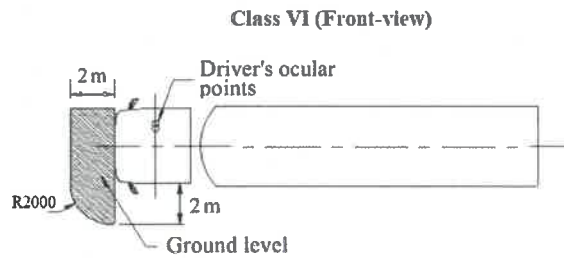
Figure 11 – Minimum required fields of vision for goods vehicles over 3.5 tonnes maximum mass (note: class VI is optional for goods vehicles \leq 7.5 tonnes) (source: adapted (for right-hand-drive) from UN R46)
